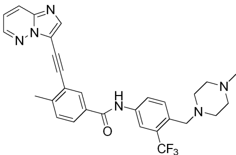
Ponatinib, Lot 02, NMR in DMSO
