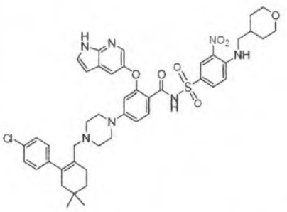
ABT-199, Lot 09, NMR in DMSO
