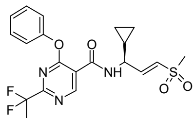
VVD-214, Lot 01, NMR in DMSO-D 2 O
