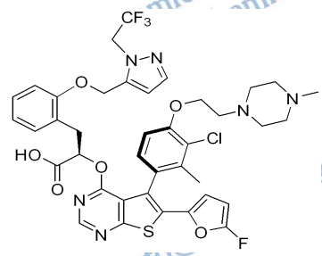
S63845, Lot 04, NMR in d6-DMSO
