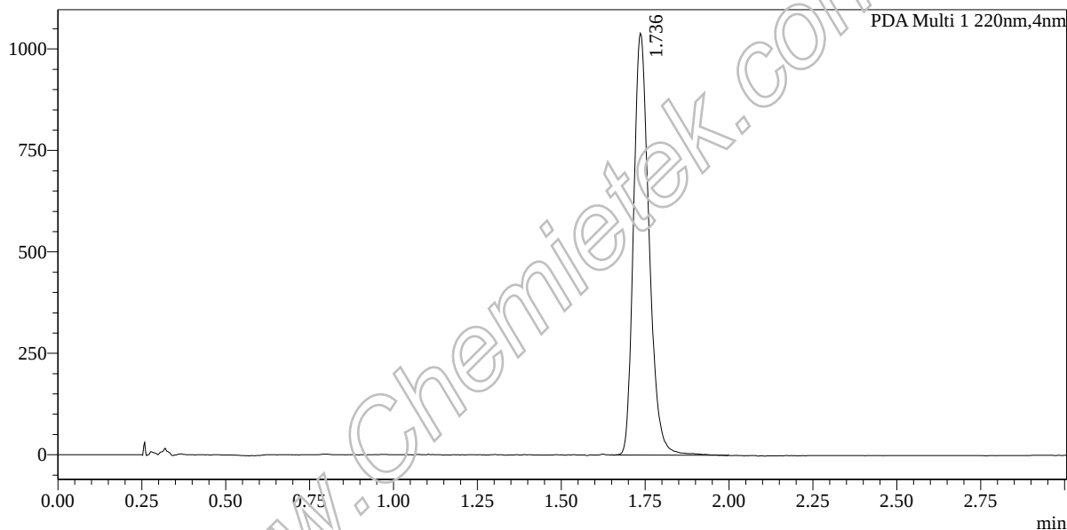
Chromatogram
