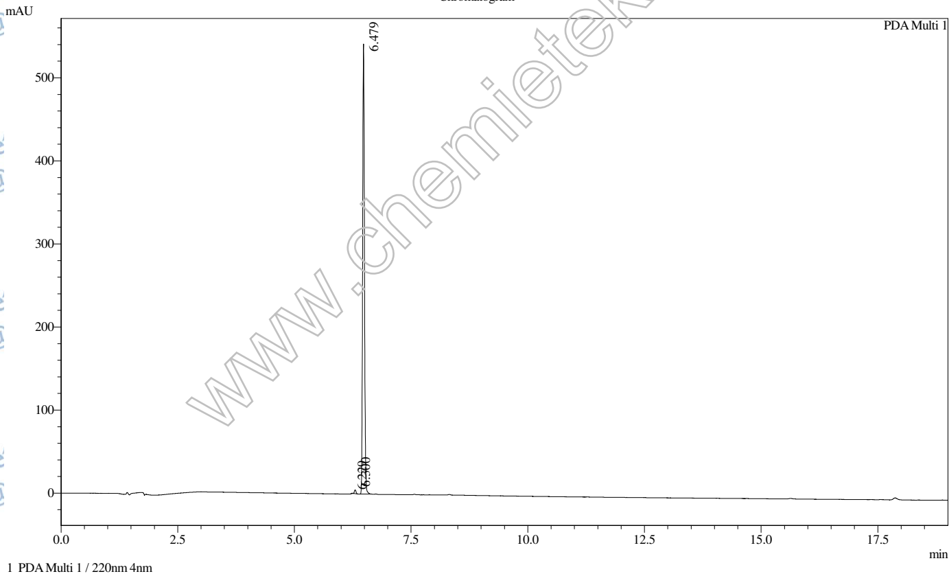
Chromatogram
