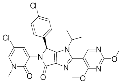
NVP-HDM201, Lot 01, NMR in d6-DMSO
