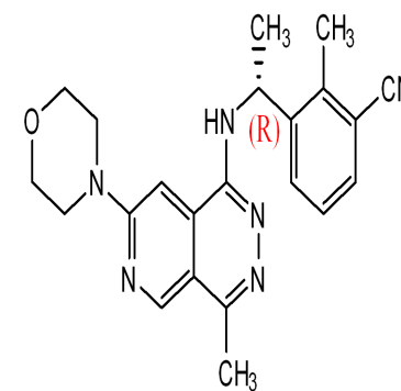
MRTX0902, Lot 01, NMR in DMSO
