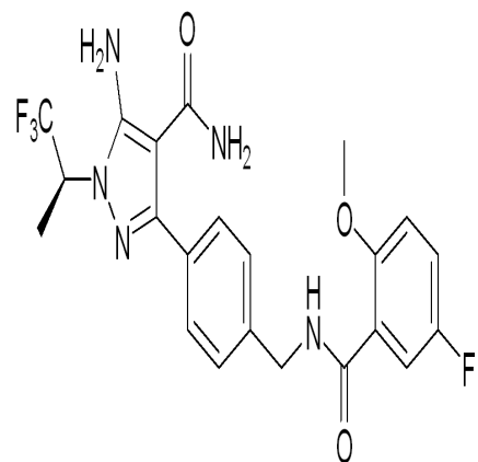
Pirtobrutinib (LOXO-305), Lot 01, NMR in DMSO
