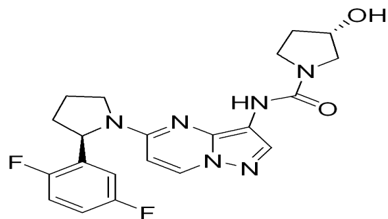
LOXO-101 (Larotrectinib), Lot 01, NMR in DMSO
