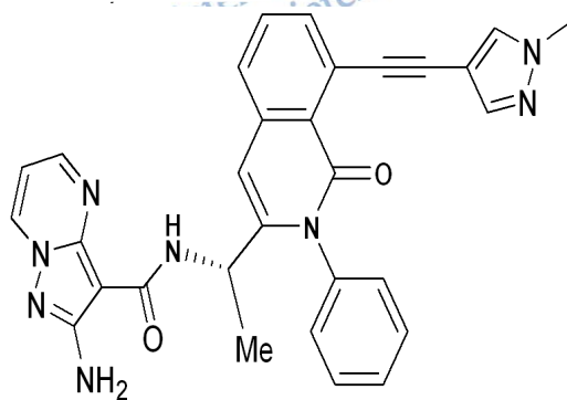
IPI-549, Lot 02, NMR in d 6 -DMSO
