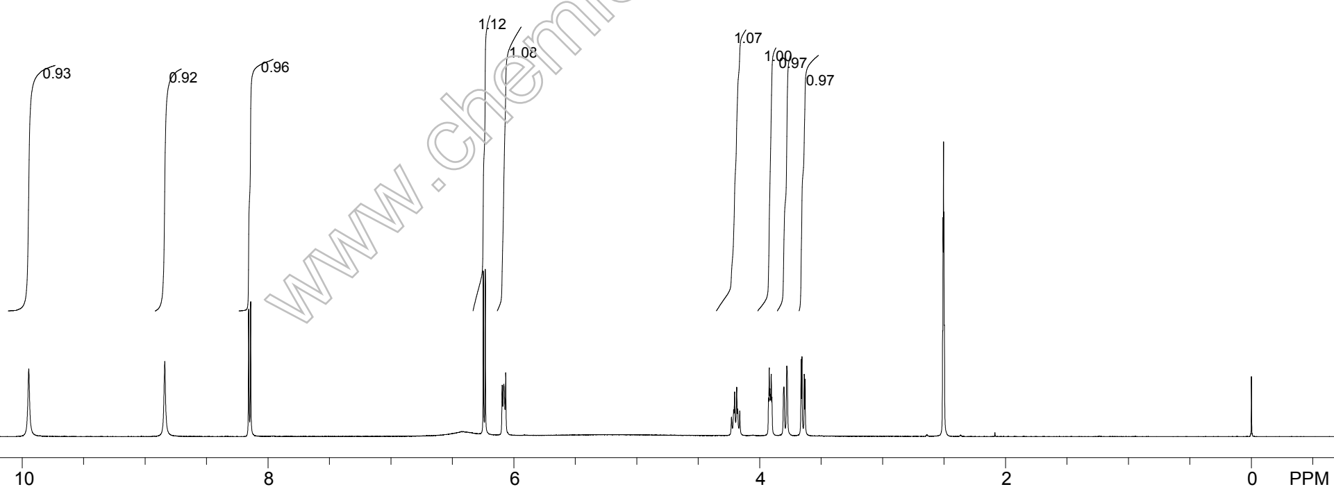
Gemcitabine HCl Salt, Lot 01, NMR in d6-DMSO
