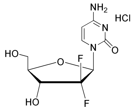
Gemcitabine HCl Salt, Lot 01, NMR in d6-DMSO
