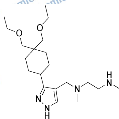
GSK3368715, HCl Salt, Lot 01, NMR in D2O
