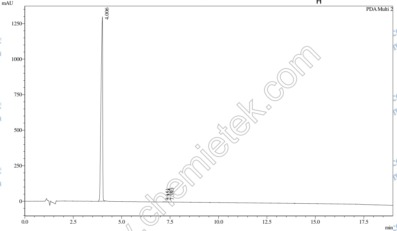
Chromatogram
