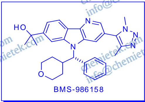
BMS-986158, Lot 02, NMR in DMSO
