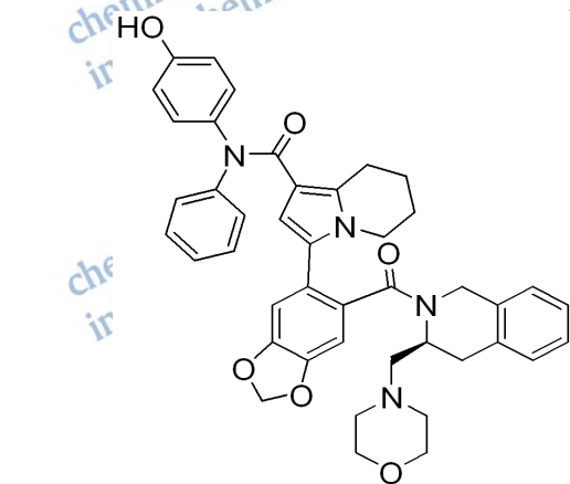
BCL-201 (S55746), Lot 01, NMR in d6-DMSO
