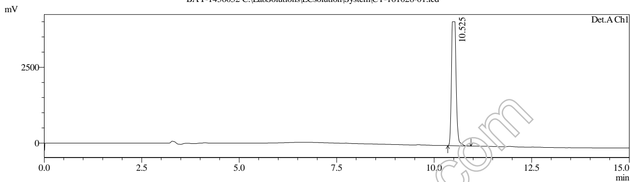
LC Chromatogram BAY-1436032 C:\LabSolutions\LCsolution\System\CT-161028-01.lcd
