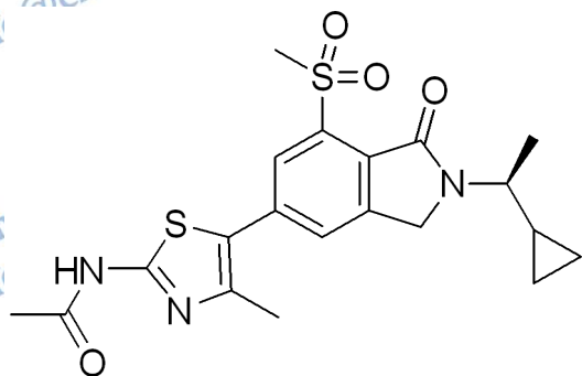
AZD3458, Lot 01, NMR in d6-DMSO
