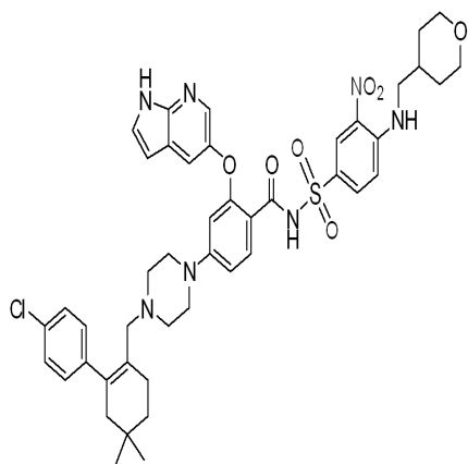
ABT-199, Lot 11, NMR in DMSO
