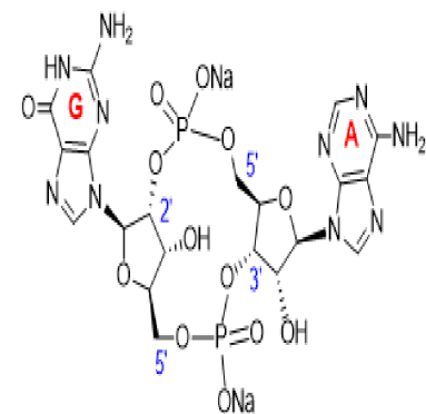
2', 3' - cGAMP Sodium, Lot 05, NMR in D2O
