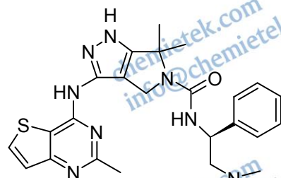
PF-03758309, Lot 04, NMR in MeOD
