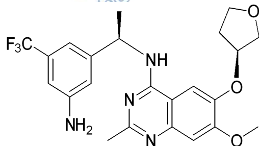
BI-3406, Lot 01, NMR in CDCl 3
