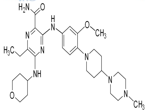
Gilteritinib, Lot 08, NMR in d4-MeOH
