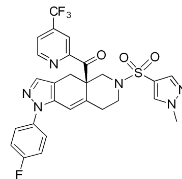
CORT-125134, Lot 01, NMR in CDCl 3
