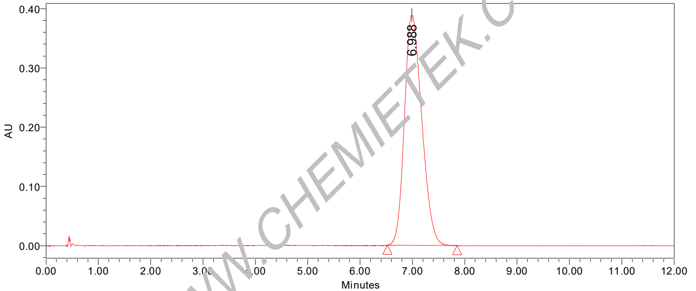
Auto-Scaled Chromatogram
